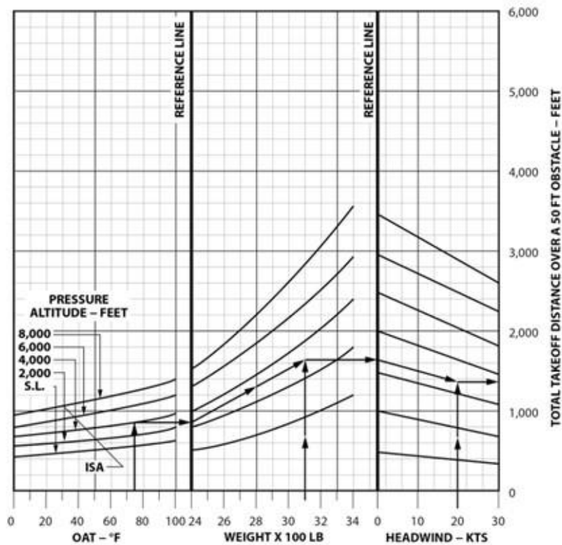
Figure 32. Obstacle Take-off Chart
