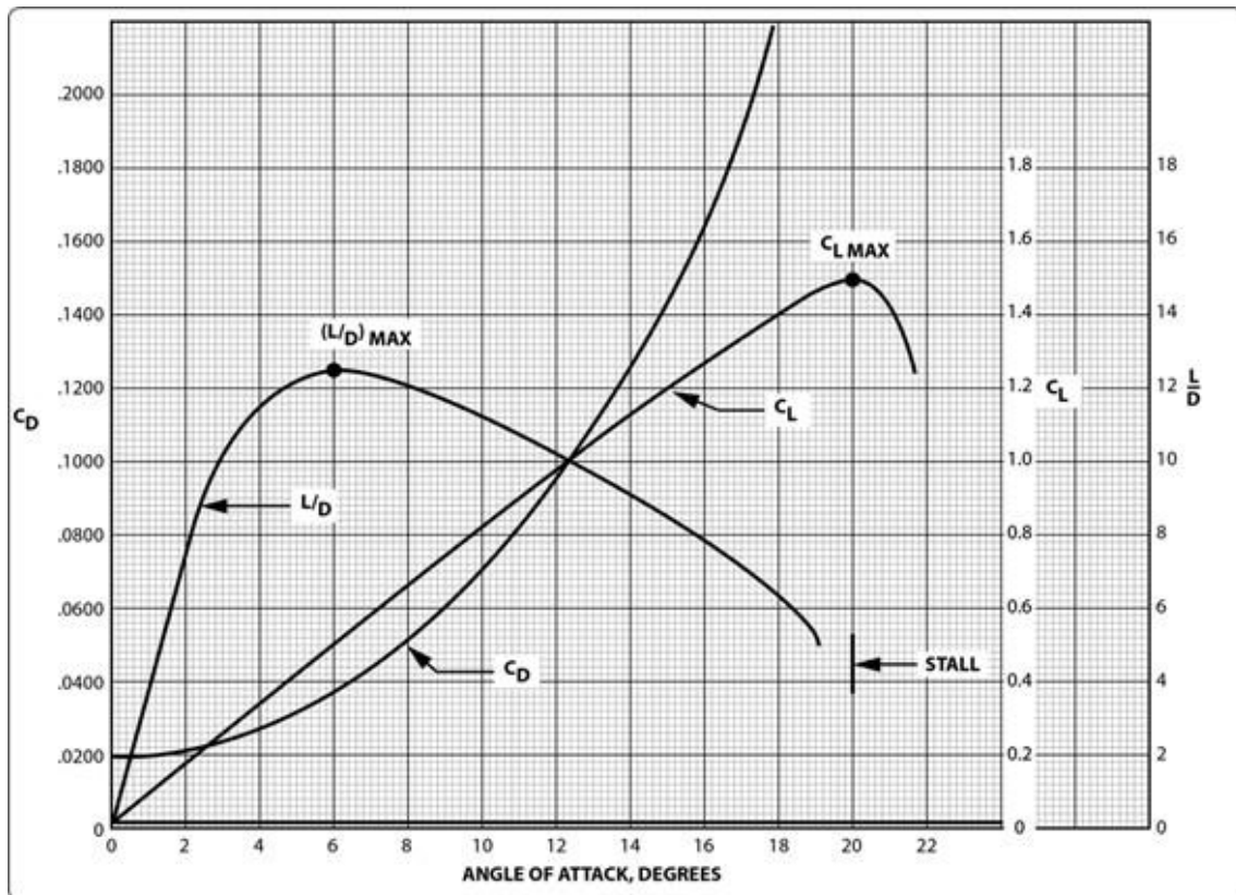
Figure 3. Angle of Attack vs. Lift
