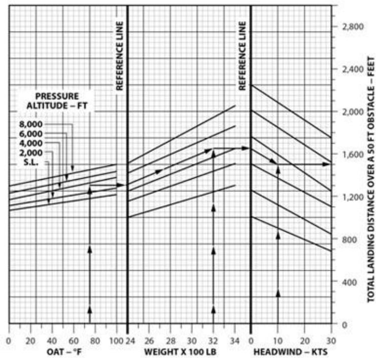
Figure 35. Normal Landing Chart
