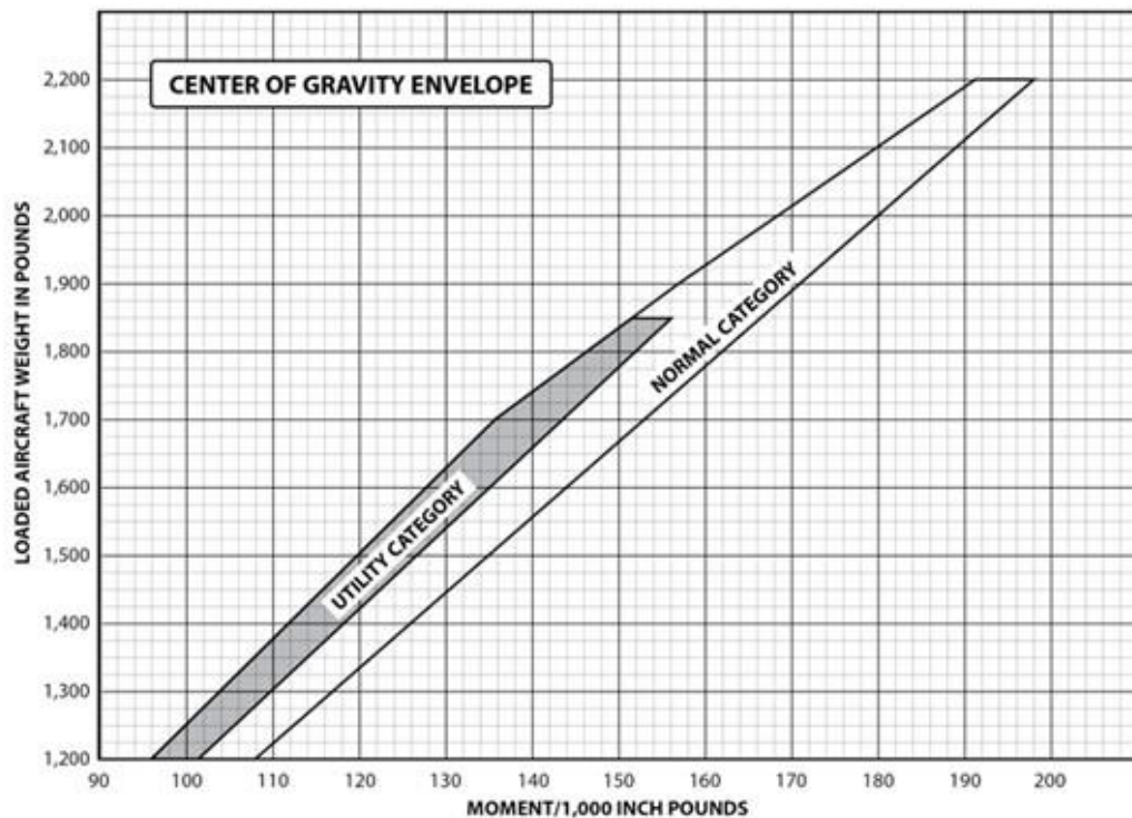
Figure 38. Loading Graph and Center of Gravity Envelope
