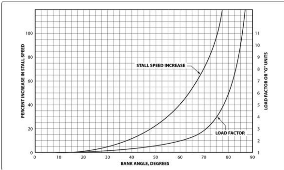
Figure 4. Stall Speed vs. Load Factor
