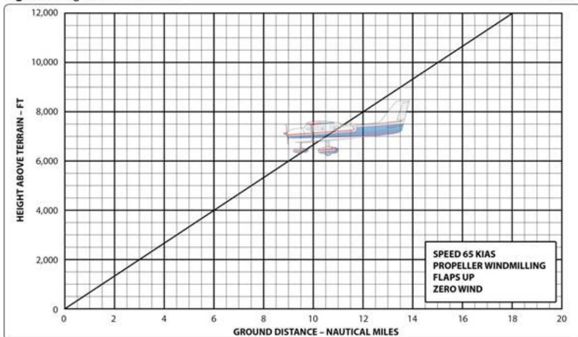
Figure 3A. Maximum Glide Distance
