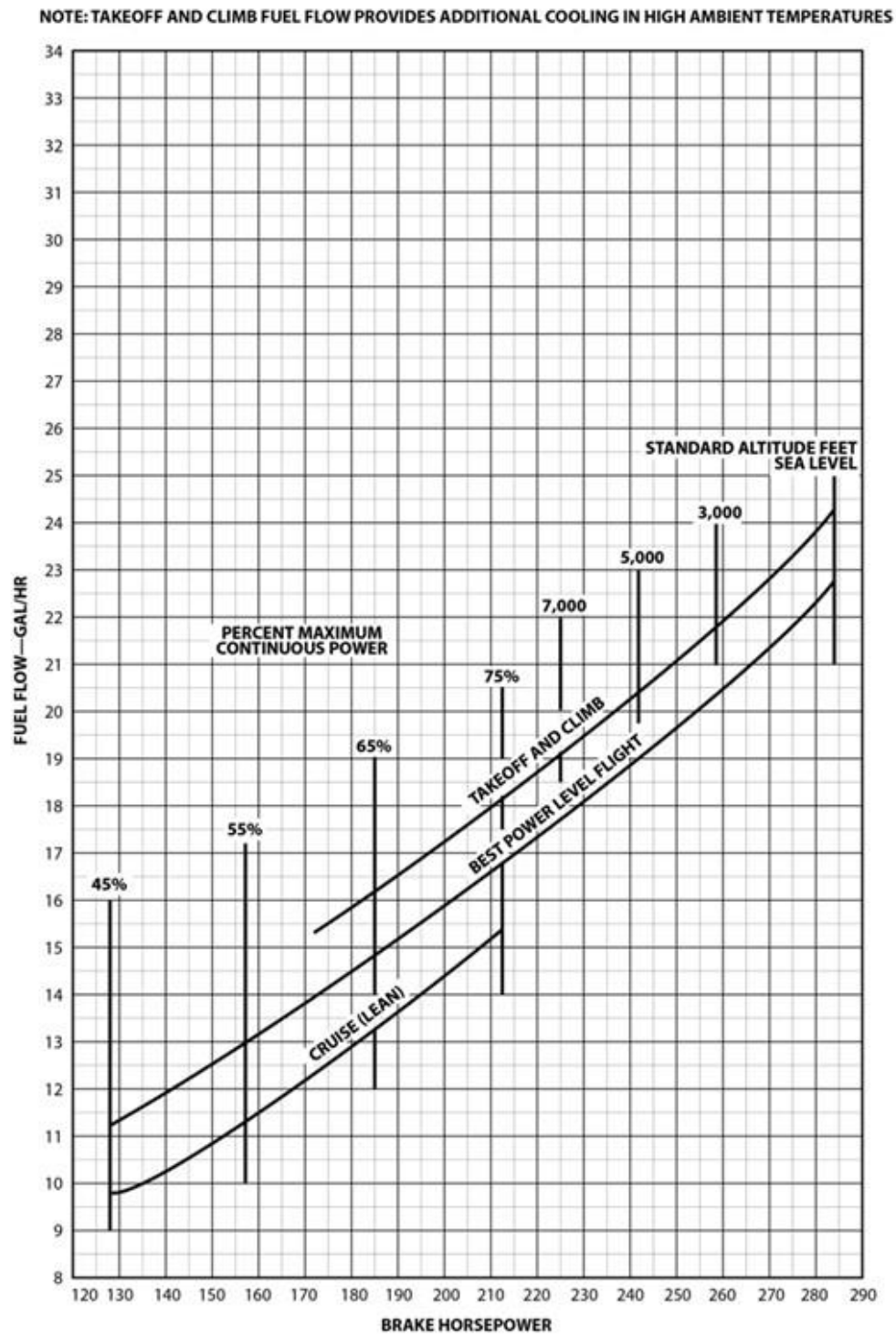
Figure 8. Fuel Consumption vs. Brake Horsepower
