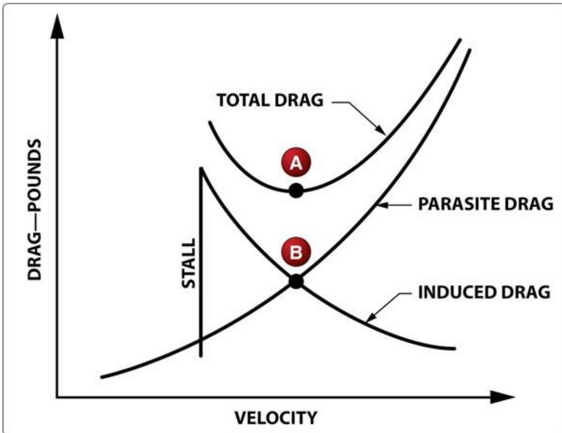
Figure 1. Drag vs. Velocity
