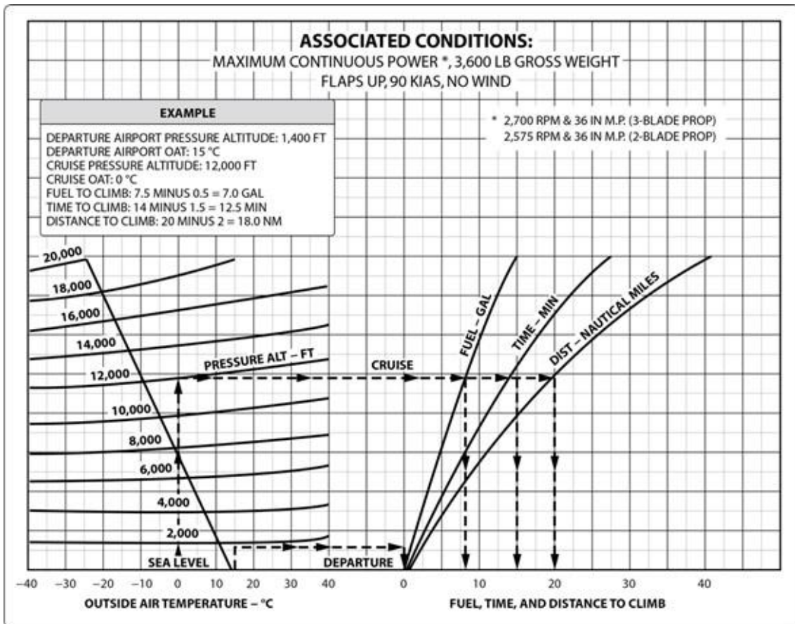
Figure 15. Fuel, Time, and Distance to Climb
