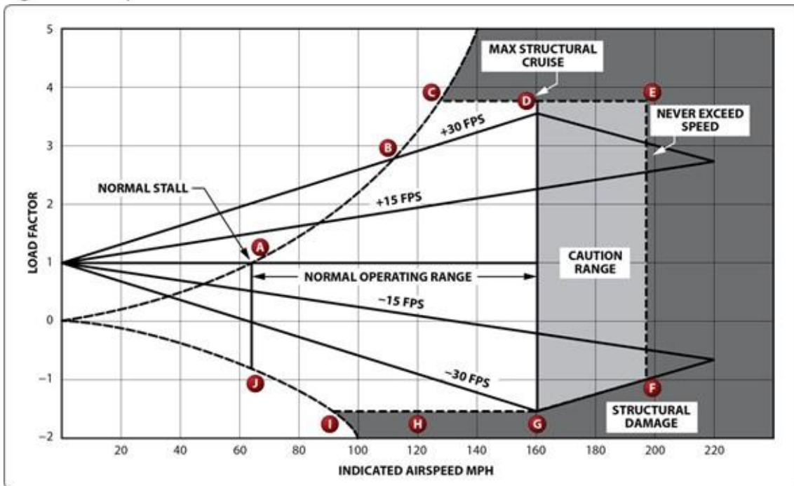
Figure 5. Velocity vs. Load Factor
